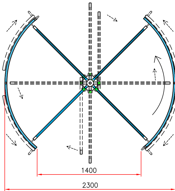
REVOLVING MA 2300
